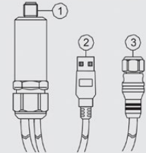
Connection of Programming Adapter MPI-200.
